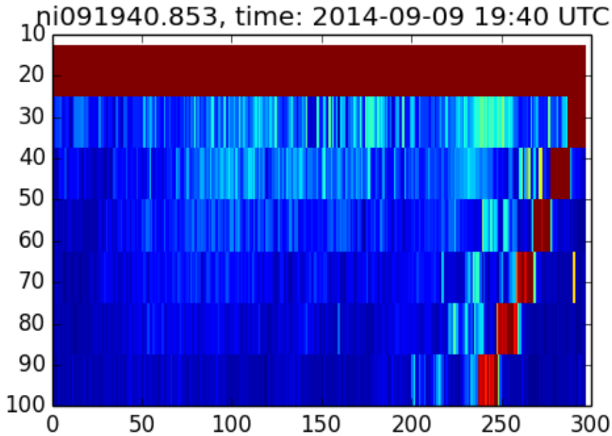
Figure 4. Acoustic returns from the 300 kHz echosounder equipped OTN glider in Roseway Basin, from 19:40 UTC on Sept 9, 2014. The x-axis shows the ping count (the echosounder pinged every 4 seconds) and the y-axis shows the range in meters beneath the glider. Just before ping 250, the glider observed a return from the seabed (at 100-m range; i.e. the glider was 100 m off the bottom) and as it continued its dive, the seabed return was observed at closer and closer ranges until the end of the dive.
